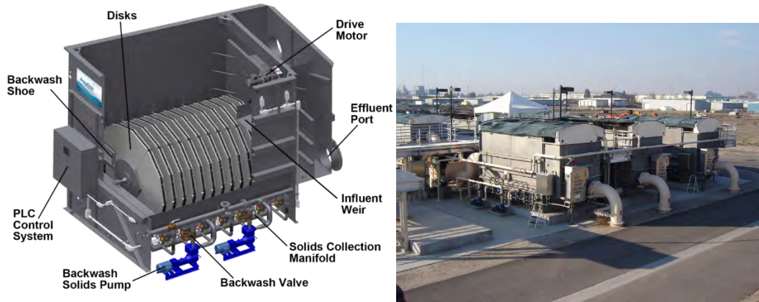
Figure 5.3 Configuration of Basic Disk Filter
