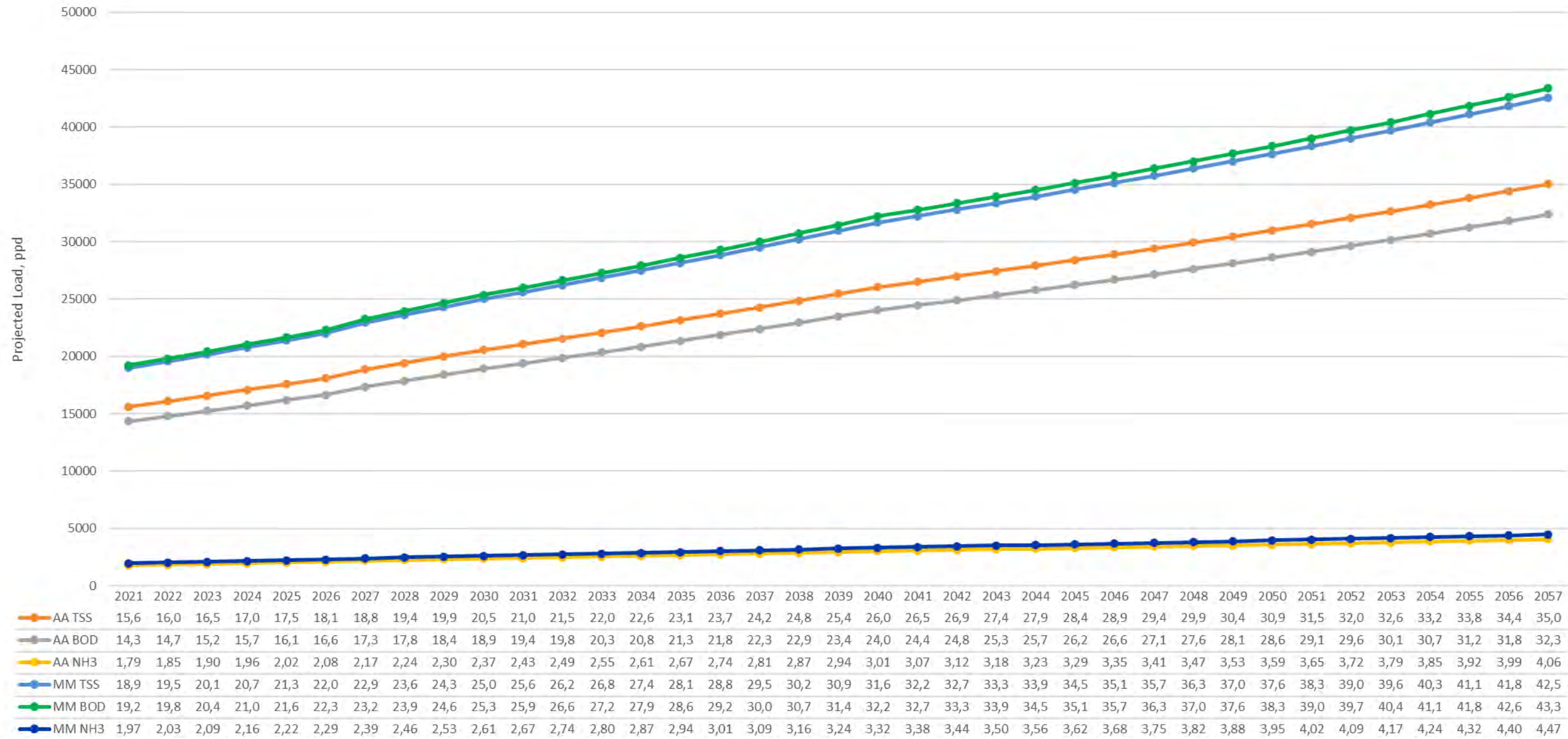
Figure 2.16 Projected Loads
